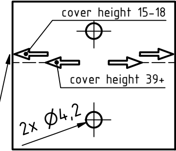
drilling template (1 : 1)
